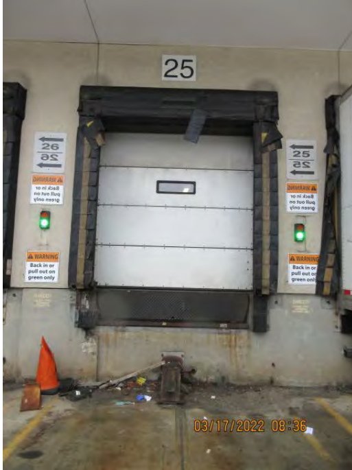
DOOR 25 Remove Existing TRS and Install Star 4 Truck Restraint
