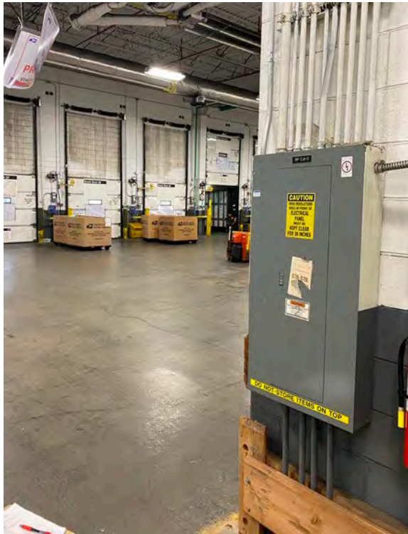
DOORS 18-33 Panel RPC.6-2 Add New 1 Pole 20A Circuit Breaker (1 for every 4 Doors)
